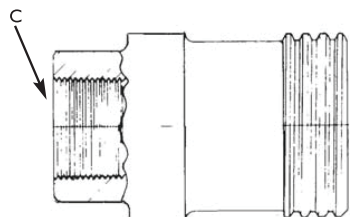
FIXED END FNPT
